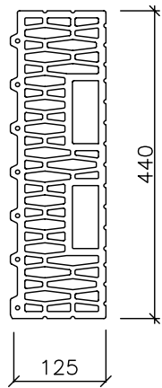
POROTHERM 44 K 1/2 CB
