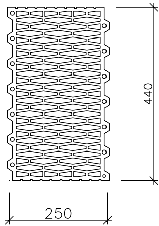
POROTHERM 44 CB
