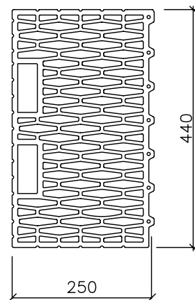
POROTHERM 44 K CB
