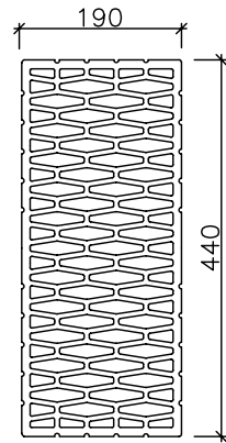
POROTHERM 44 R CB
